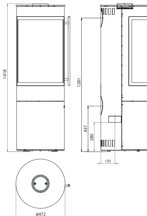
PULAR PLUS Compact
