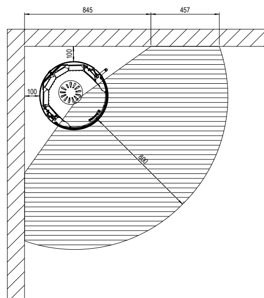
Stove installed diagonally in corner
