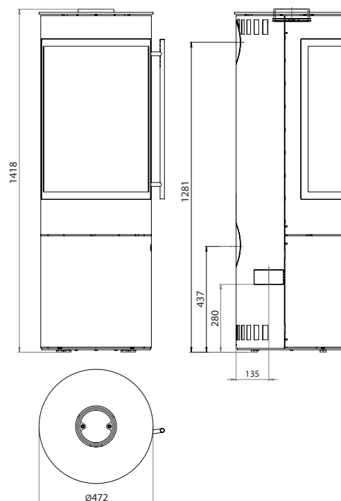
PULAR PLUS Compact
