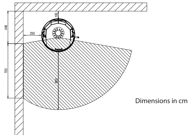
Stove installed straight in corner
