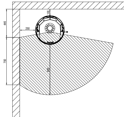
Stove installed straight in corner
