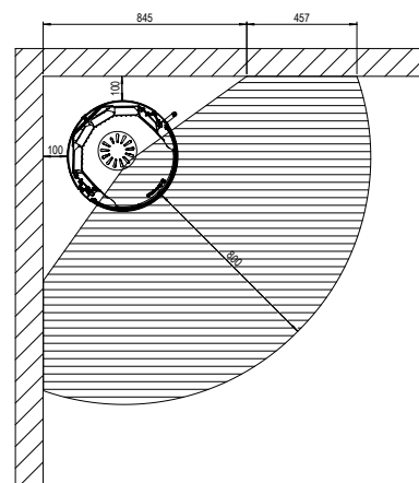
Stove installed diagonally in corner
